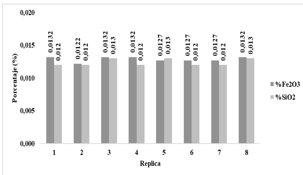
Figure 4. Experimental results in the determination of iron (III) (Fe 2 O 3 ) and silicon dioxide (SiO 2 )
