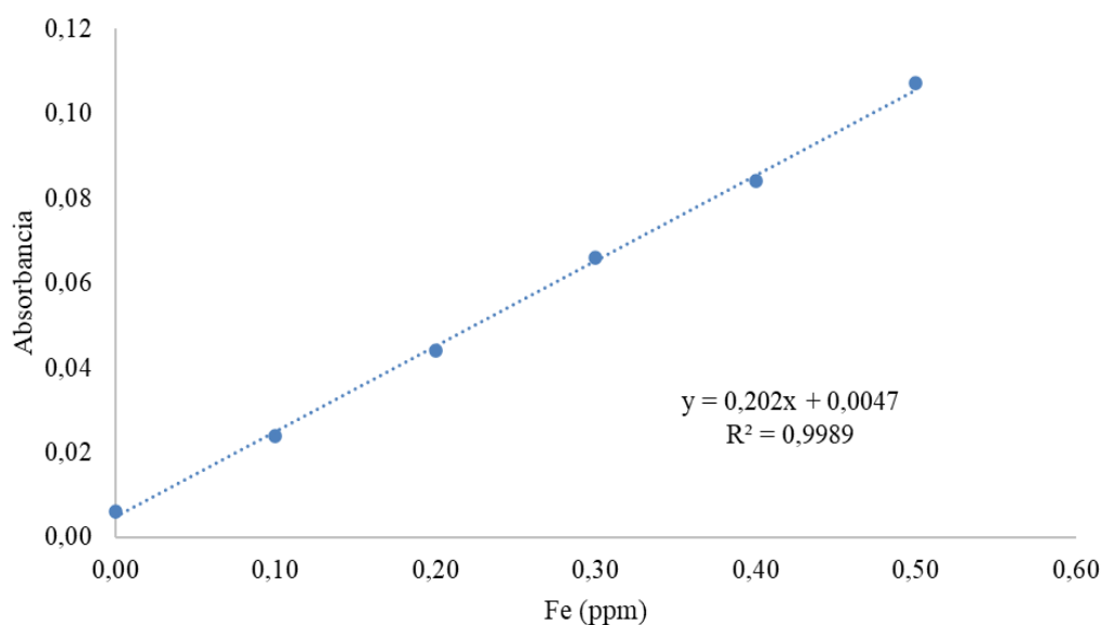
Figure 2. Calibration curve for the determination of iron (Fe)
