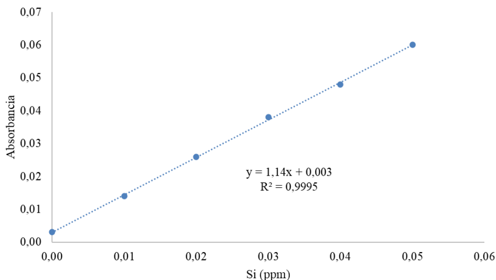
Figure 3. Calibration curve for the determination of silica (Si)
