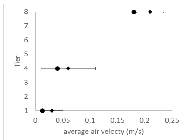
Figure 3. Experimental (diamonds) (11) and simulated (circles) air velocities in bins in different tiers. Air mass flow rate of 1,95 kg/s
