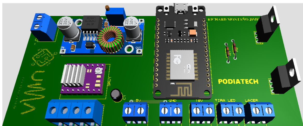
Figure 3. 3D modelling of PCB board
