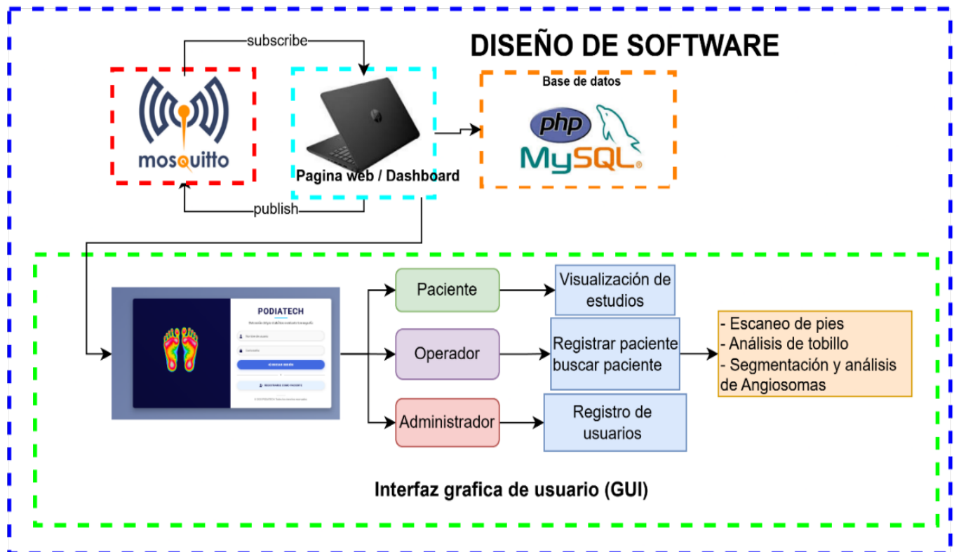
Figure 4. PODIATECH software design scheme
