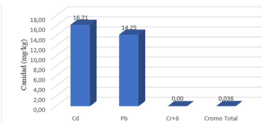
Figure 14. Heavy metal test results, point 2
