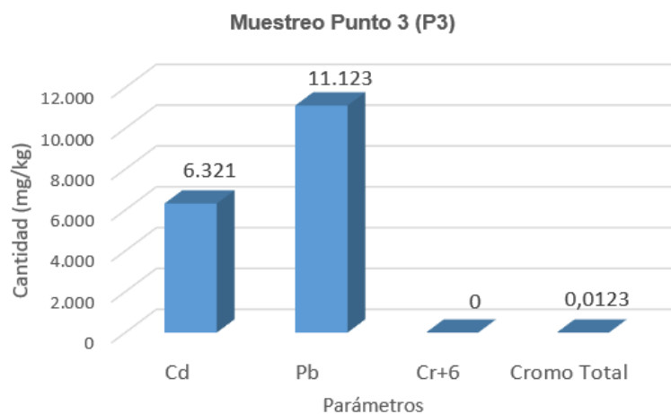
Figure 8. Heavy metal test results, point 3
