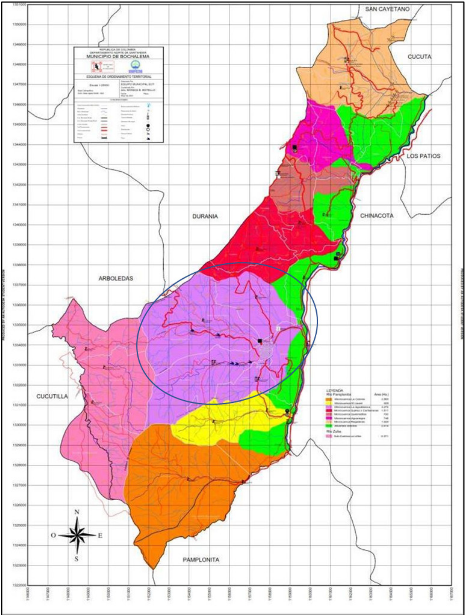
Figure 3. Hydrological Map of the Municipality of Bochalema
