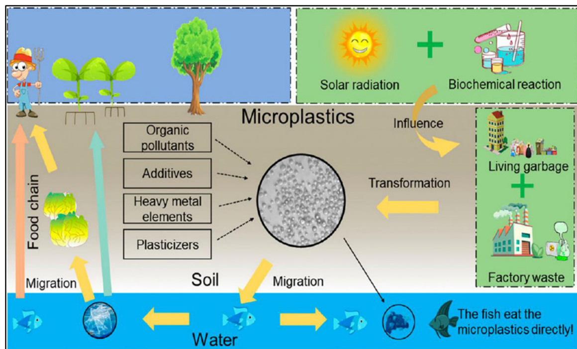
Figure 3. The origin, migration, and damage of microplastics
