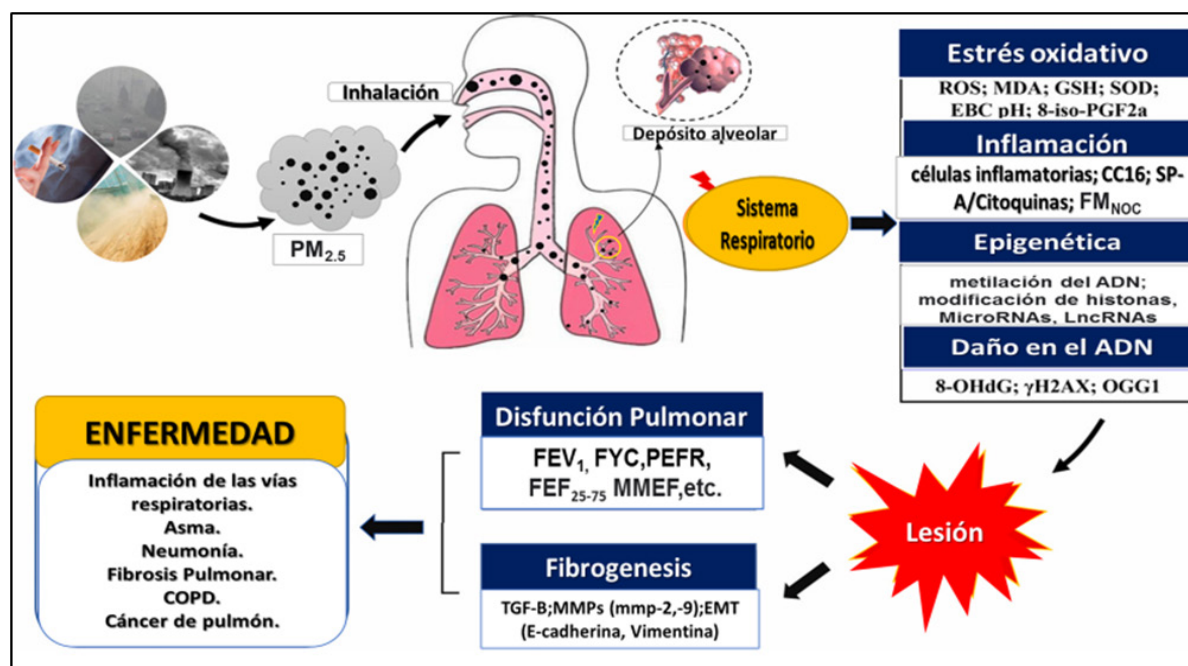
Figure 1. Effect of PM 2.5 on human health
