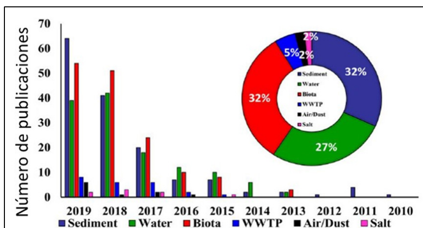
Figure 5. Results from literature using FTIR
