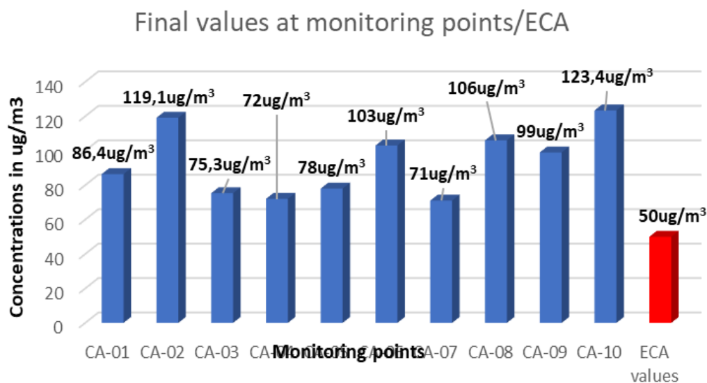
Figure 9. Final values at monitoring points compared to the ECA
